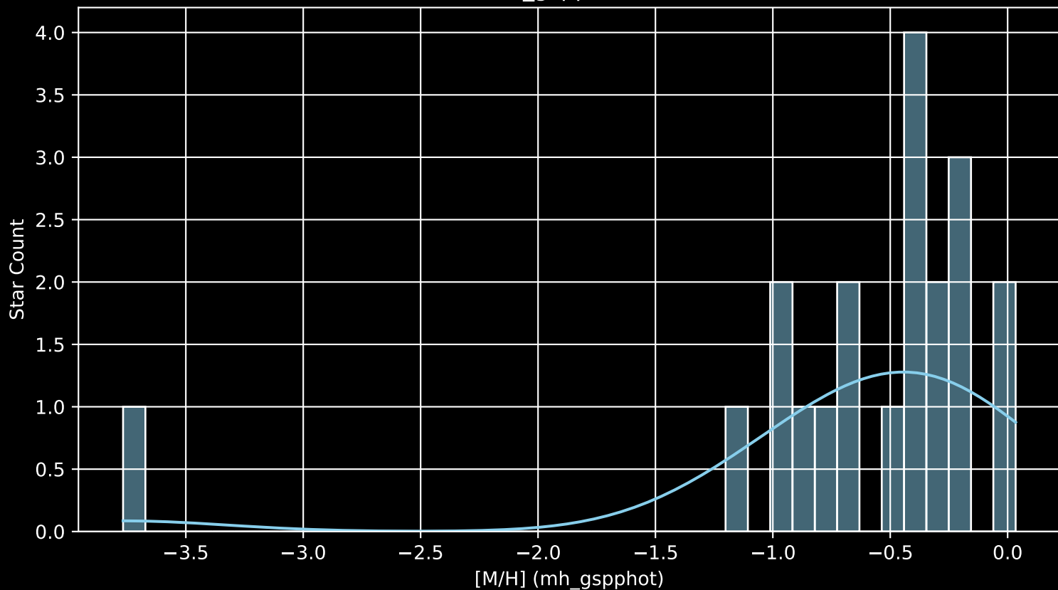
APOGEE DR17 Field: [ANDR3 [M/H] (mh_gspphot) (n= 20)
