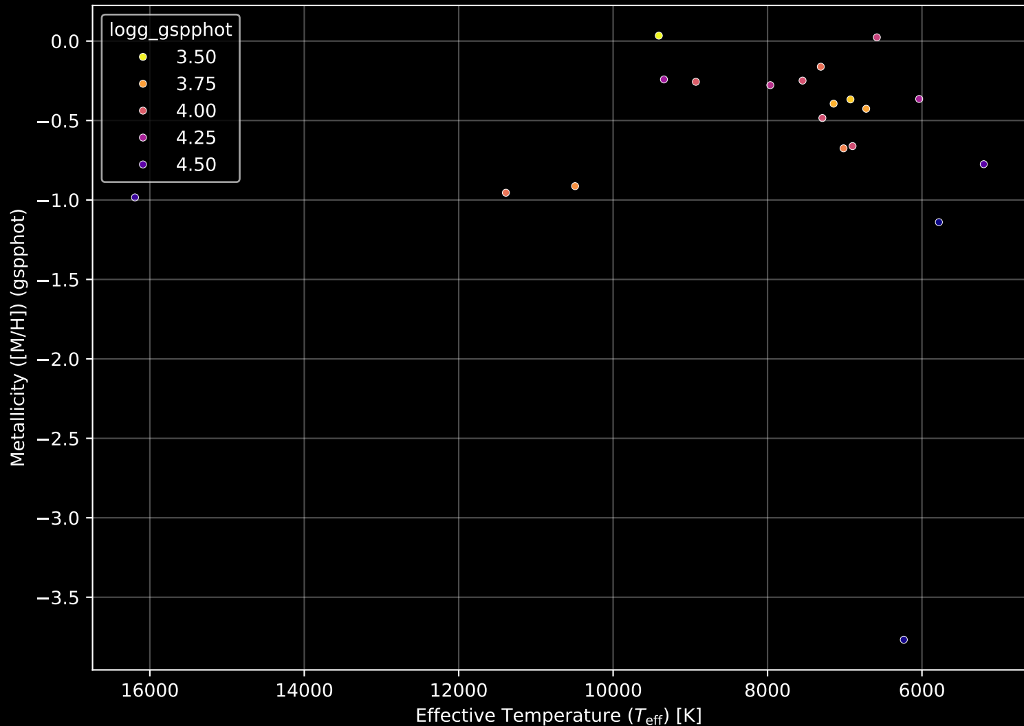
APOGEE DR17 Field: [ANDR3] Stellar Population Parameters (n= 20)
