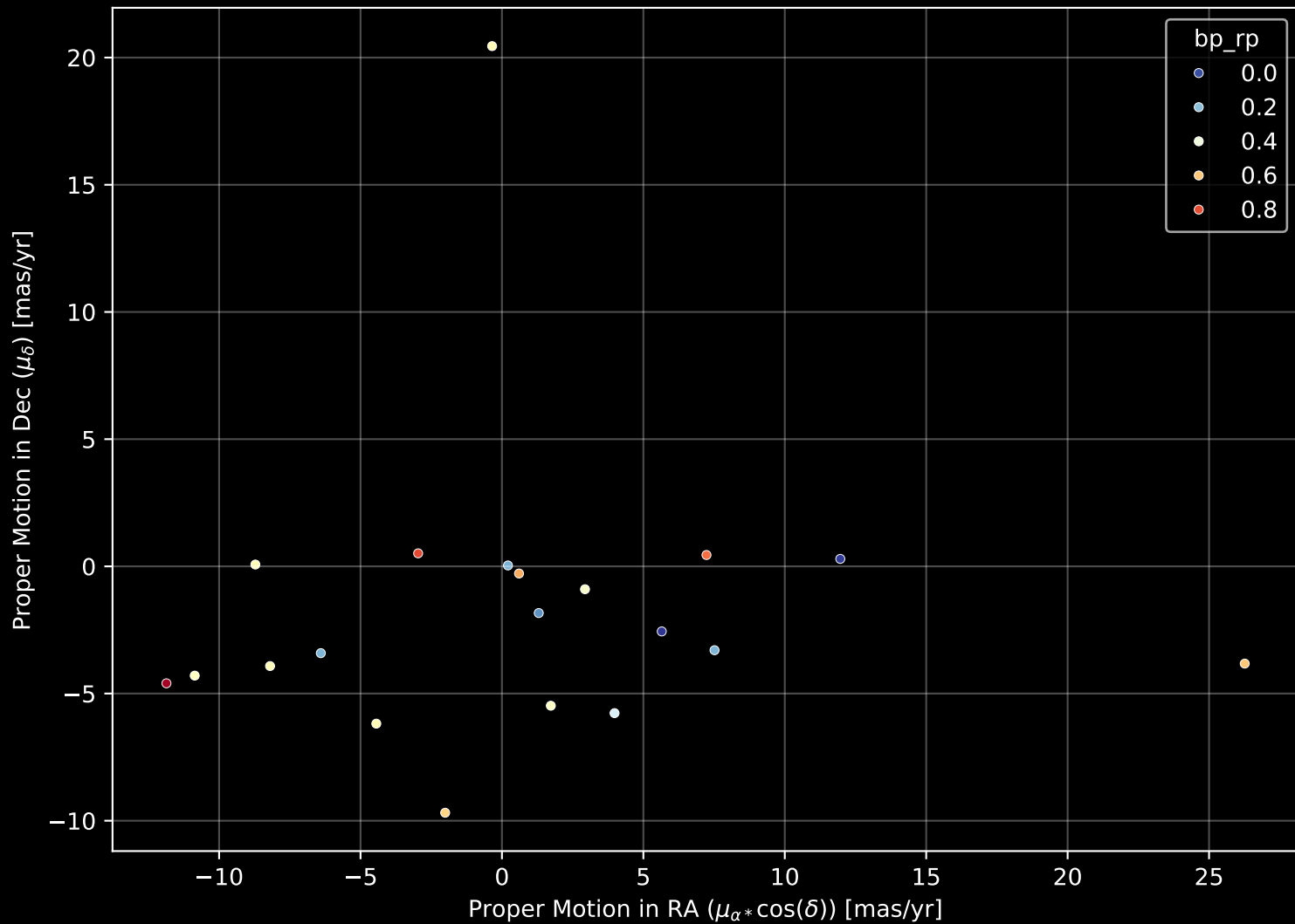
APOGEE DR17 Field: [ANDR3] Proper Motion Diagram (n= 20)
