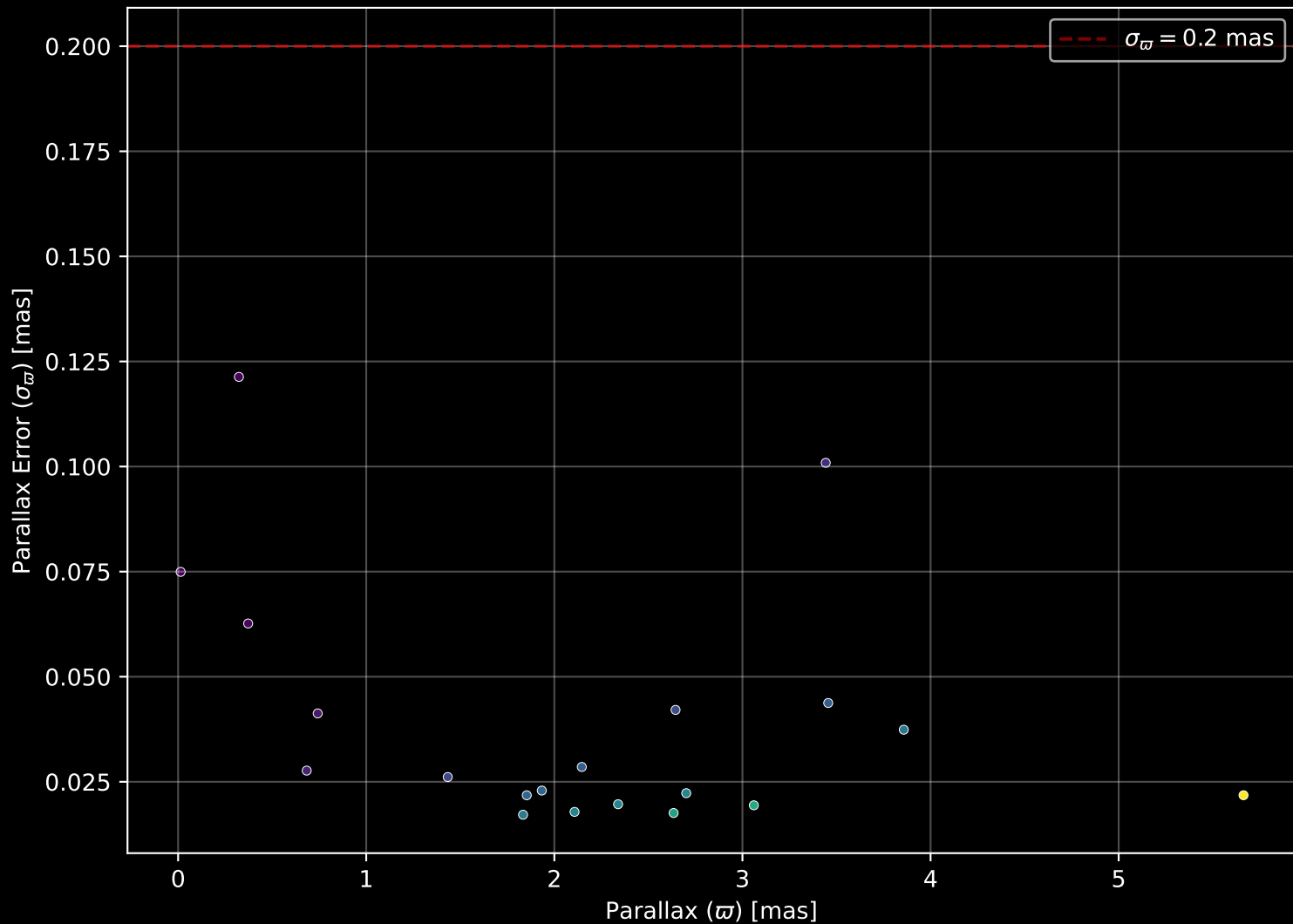
APOGEE DR17 Field: [ANDR3] Parallax Quality (n= 20)
