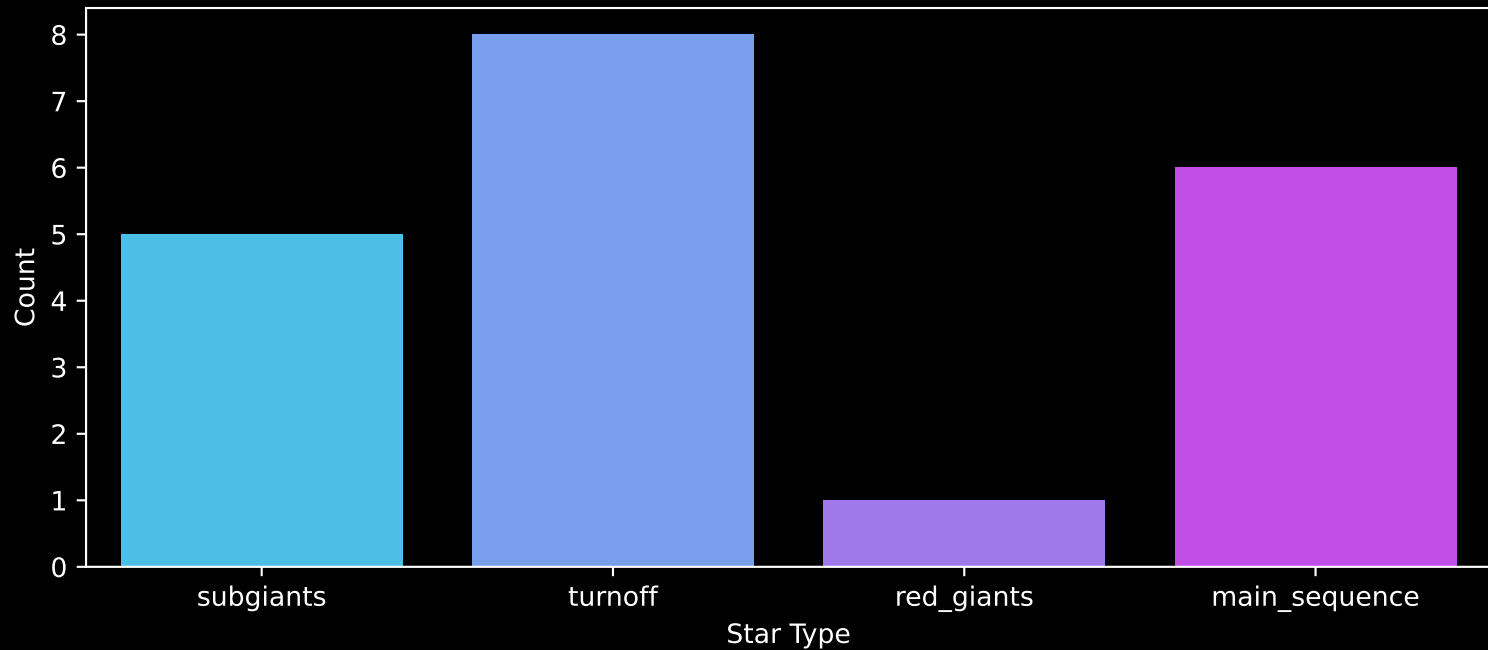
APOGEE DR17 Field: [ANDR3] Count plot of Star Type
