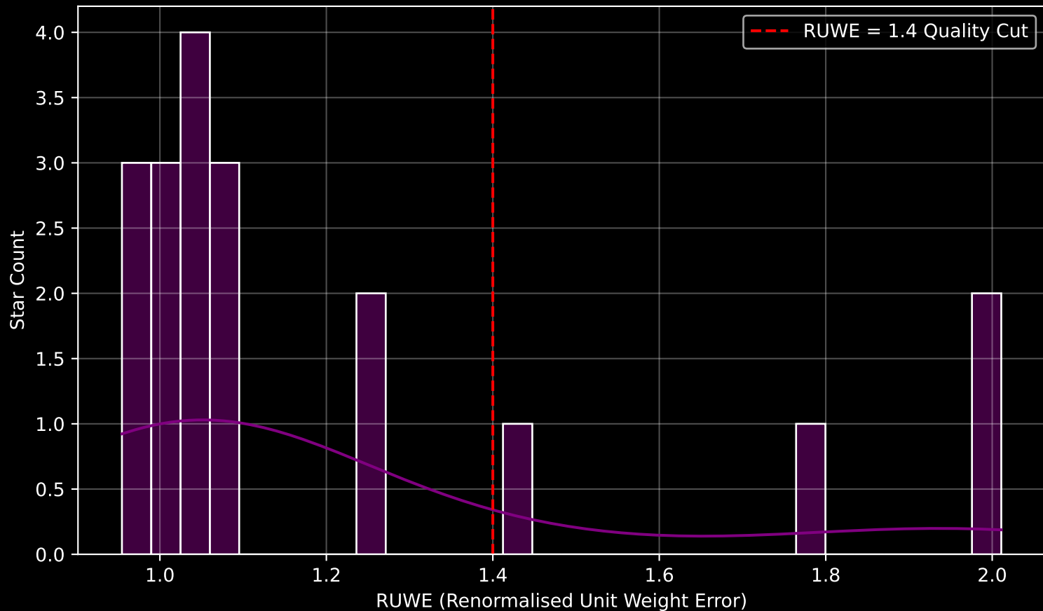
GAPOGEE DR17 Field [ANDR3] RUWE Distribution (n= 19)
